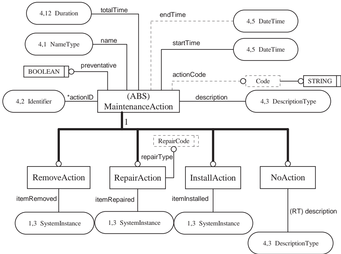
Figure B.8—SIMICA_COMMON_MODEL_DOT_99 EXPRESS-G, diagram 8 of 8
